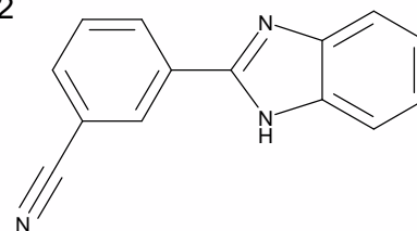
2-(3-Cyanophenyl)benzimidazole
