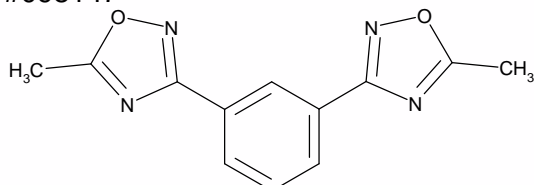
1,3-Bis(5-methyl-1,2,4-oxadiazolyl)benzene
