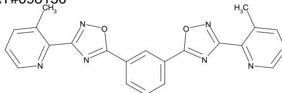
1,3-Bis[(3-(3-methyl-2-pyridin-2-yl)-1,2,4-oxadiazol)-5-yl]benzene
