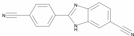
2-(4-Cyanophenyl)benzimidazole-6-carbonitrile
