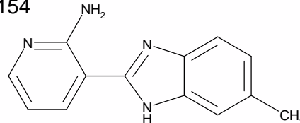
2-(2-Amino-3-pyridyl)-6-methylbenzimidazole
